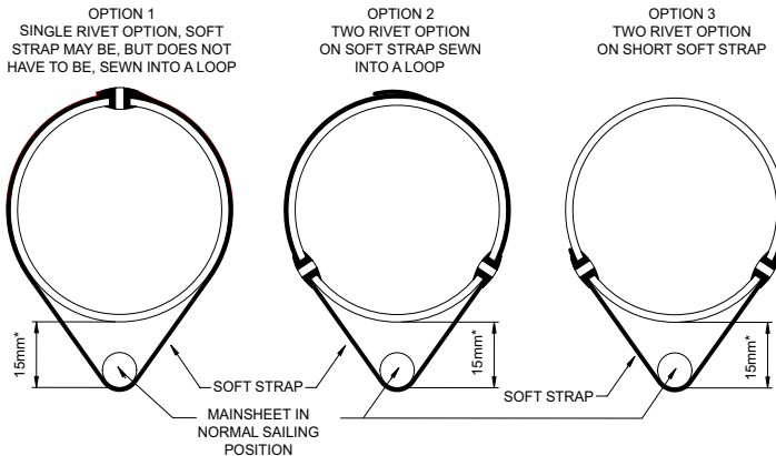
CROSS SECTIONS THROUGH BOOMS AND SOFT STRAPS SHOWING THE ONLY LEGAL FIXING OPTIONS
